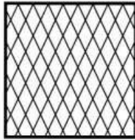
G 3 19 x 19 Outer Tube Frame Wire Diameter 5mm Aperture 50 x 100
