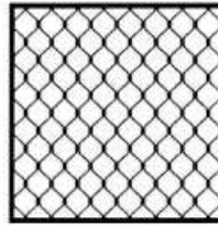
G 4 19 x 19 Outer Tube Frame Wire Diameter 5mm Aperture 56 x 65
